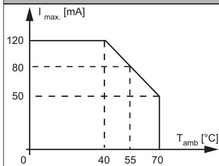
(2) BWU3164, BWU3802 Derating power supply of attached sensors
