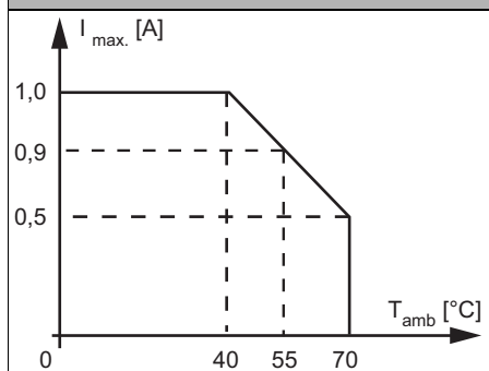
(6) BWU3890, BWU3893 Derating power supply of attached sensors
