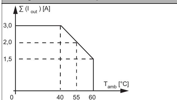
(3) BWU3317, BW3507, BWU3555, BWU3785 Derating total current of outputs
